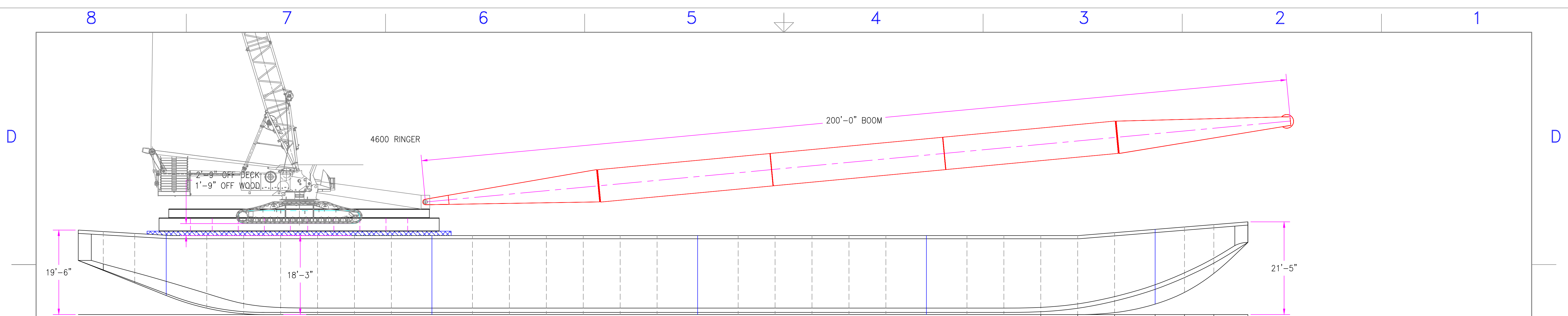
PROFILE
